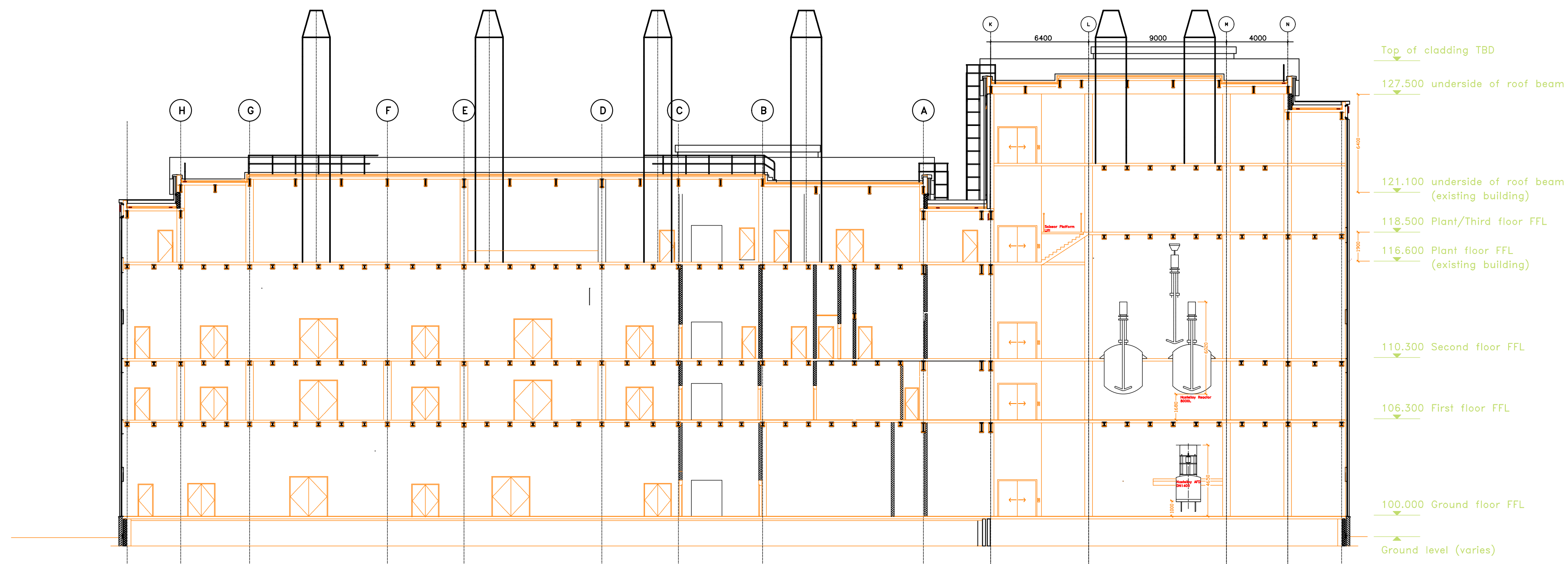
TYPICAL LONGITUDINAL SECTION THROUGH CENTRAL CORRIDOR
